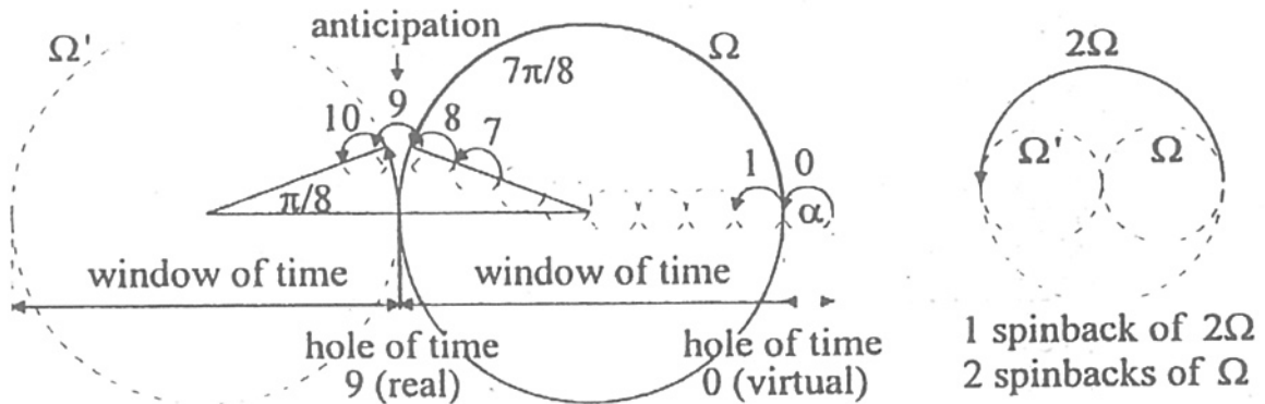
Fig. 2 : initial time flow (temporal holes and windows of the initial horizon \Omega )
