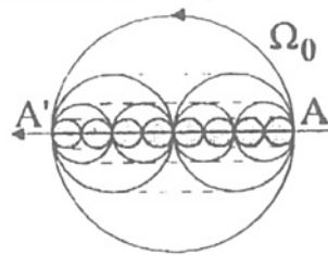
Fig. 1c : radial virtual path
