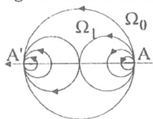
Fig. 1b : spinback of \Omega_0
