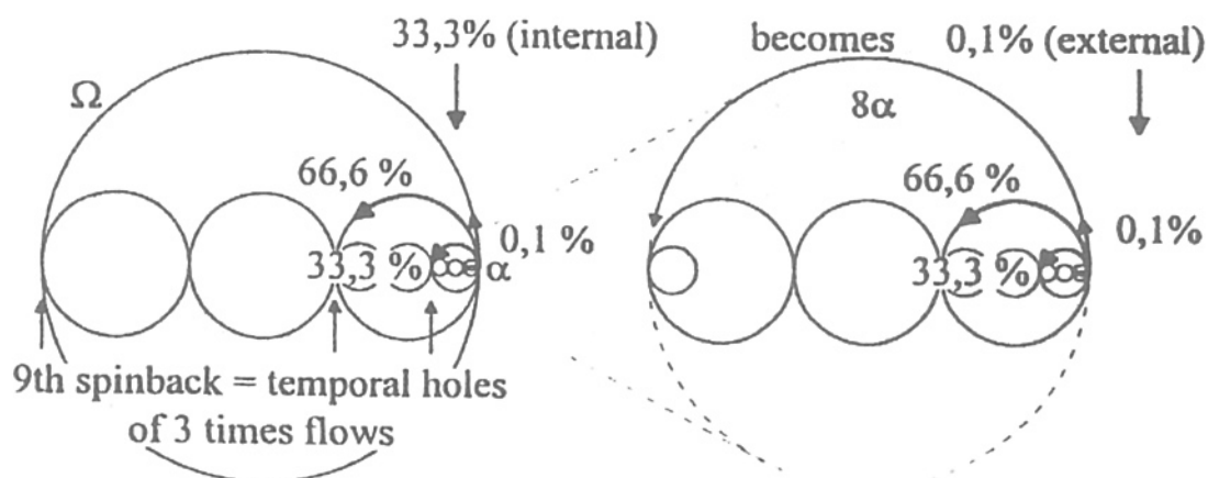
Fig. 5 : gravitation (33,3%) of \alpha in \Omega becomes the doubling energy (0,1%) of 8\alpha .
