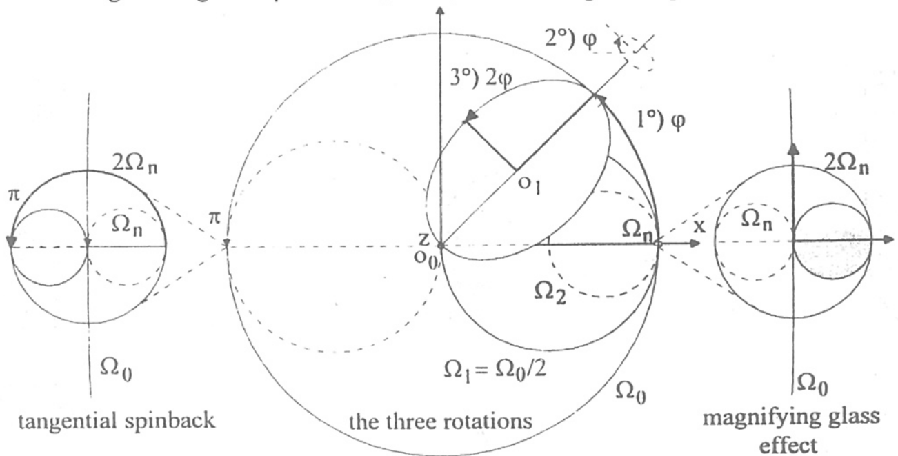
Fig. 1a : the fundamental motion or spinback.
