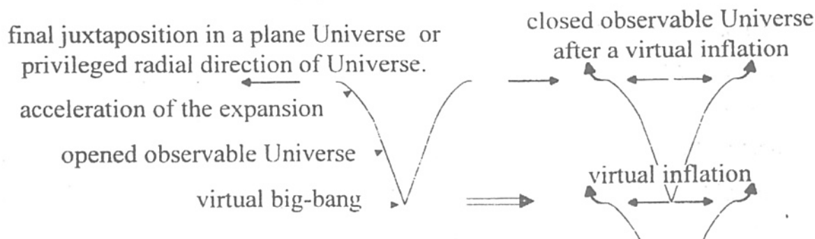
Fig. 8 : the initial and final cyclic juxtapositions of the doubled embedded Universes.
